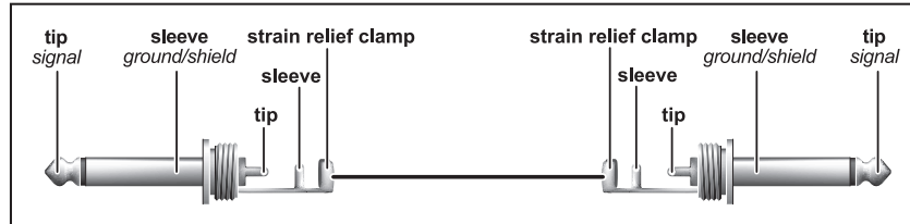
Fig. 10.1: Unbalanced 1/4" cable with 1/4" TS plugs
