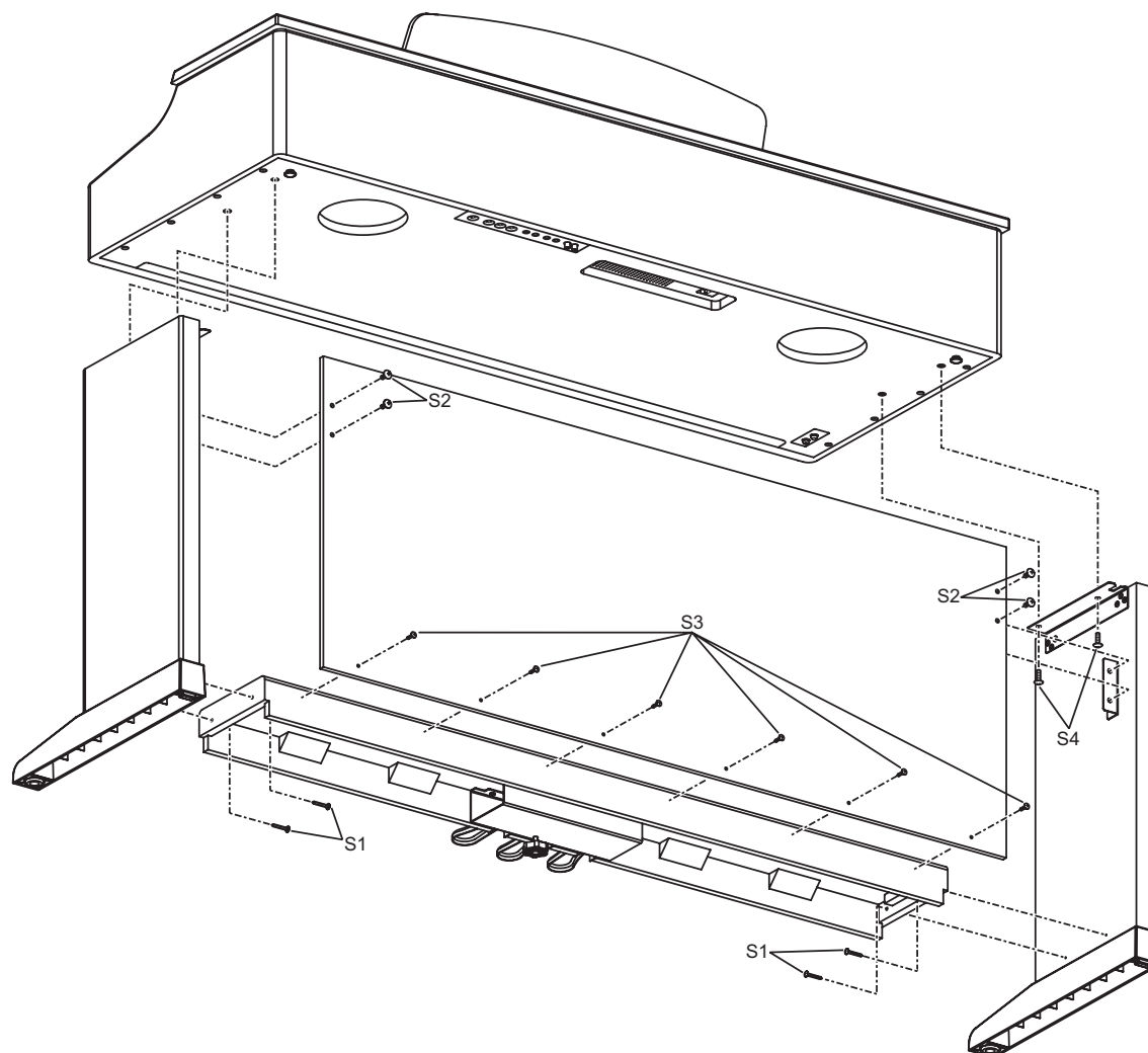
Fig. 2.2: Assembling the EG2080
