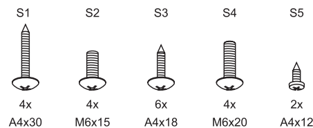
Fig. 2.1: Parts and screws for the EG2080
