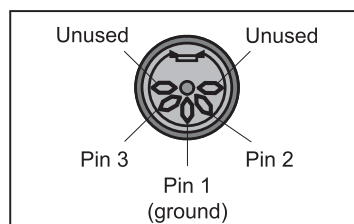
Fig. 10.4: MIDI plug pin assignment
