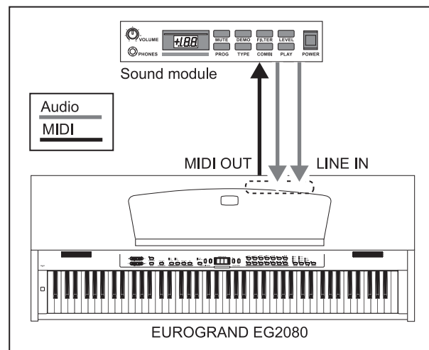
Fig. 7.3: Controlling external MIDI sound modules
