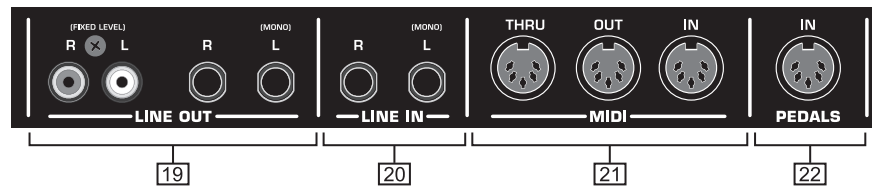
Fig. 4.2 Connectors of the EG2080
