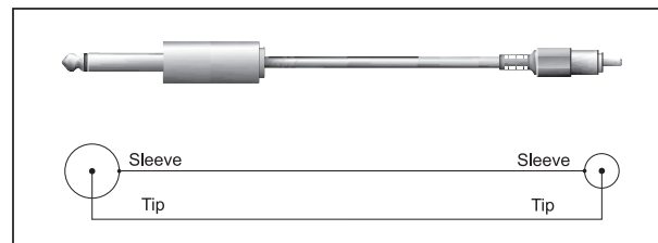
Fig. 10.3: 1/4" to RCA cable
