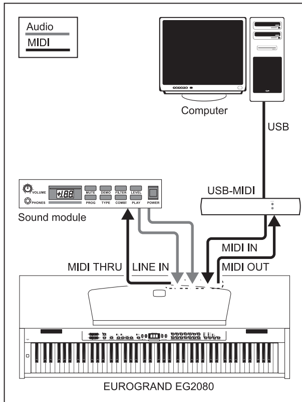
Fig. 7.4: MIDI set-up including a sequencer and external sound module
