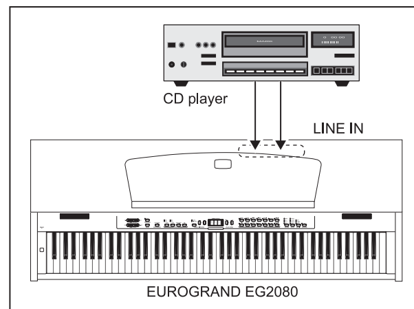
Fig. 7.1: Connecting external signal sources
