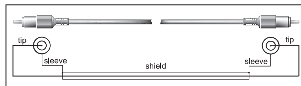
Fig. 10.2: Hi-fi RCA cable
