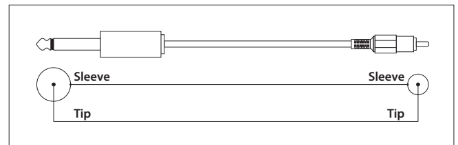
Fig. 9.3: 1/4" to RCA cable
