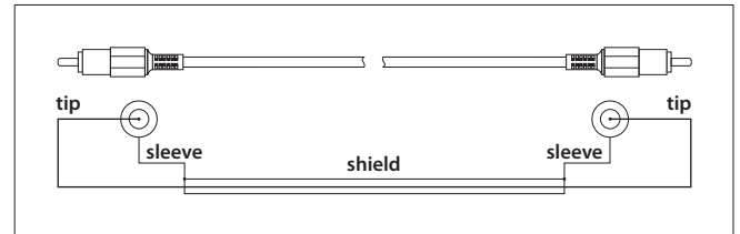
Fig. 9.2: Hi-fi RCA cable
