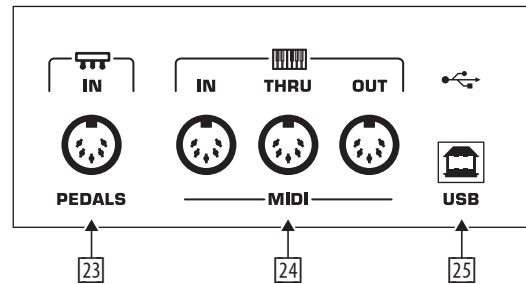
Fig. 3.2: Connectors of the EG2280USB/EG8280USB
