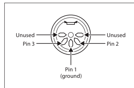
Fig. 9.4: MIDI plug pin assignment
