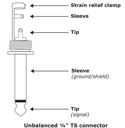
Fig. 4.3: 1/4" TS connector
