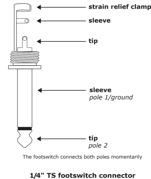
Fig. 4.1: 1/4" TS connector for foot switch
