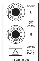
Fig. 2.5: Stereo channel inputs and LEVEL switch
