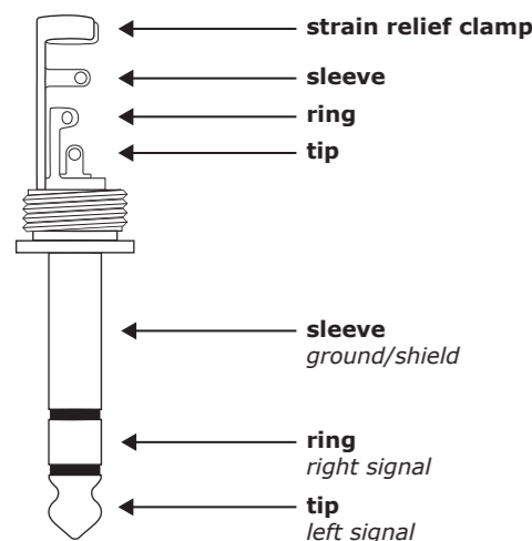
Fig. 4.4: 1/4" TRS connector
