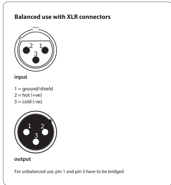
Fig. 4.2: XLR connections
