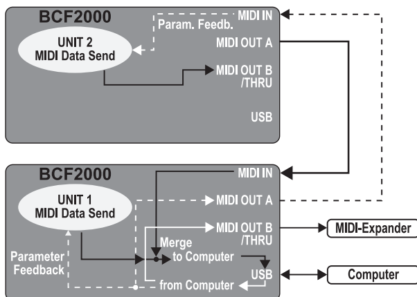
Fig. 4.4: Routing and use in USB mode 4
