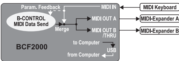
Fig. 4.5: Routing and use in stand-alone mode 1
