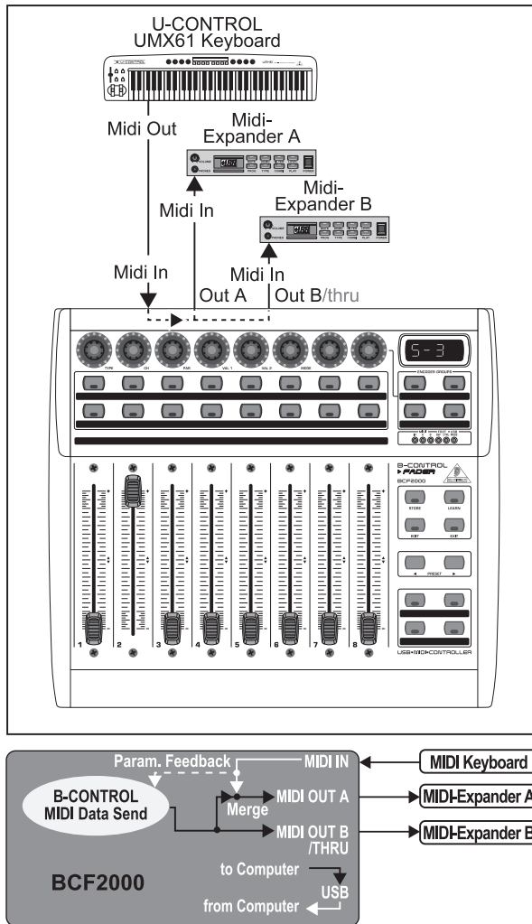
Fig. 4.7: Routing and use in stand-alone mode 3
