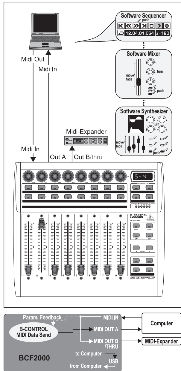
Fig. 4.8: Routing and use in stand-alone mode 4
