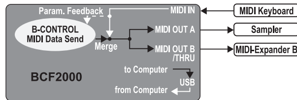
Fig. 4.6: Routing and use in stand-alone mode 2
