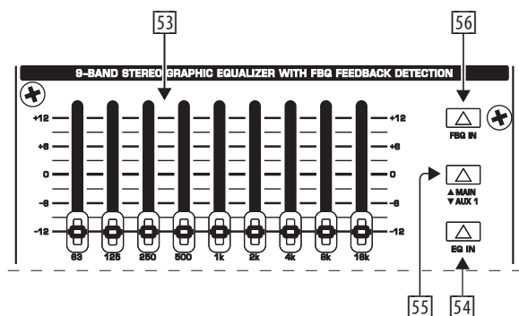
Fig. 2.24: The graphic stereo equalizer
