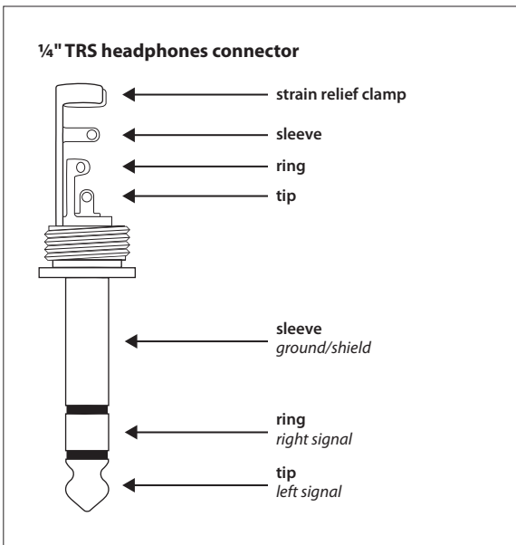
Fig. 5.6: 1/4" TRS connector for headphones
