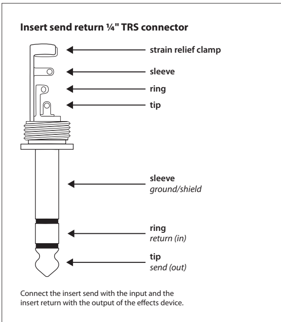
Fig. 5.7: Insert send and return 1/4" TRS connector
