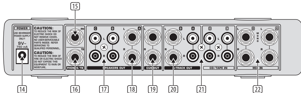
Fig. 3.2: Rear panel connectors of the MON800
