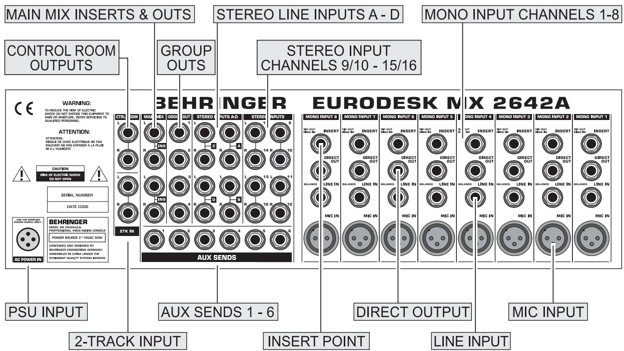
Fig. 9.2: MX2642A rear panel
