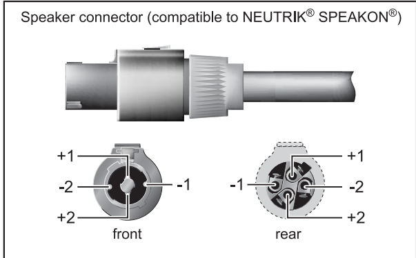
Fig. 4.5: Loudspeaker connector
