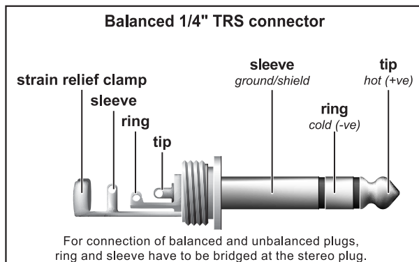
Fig. 4.2: 1/4" stereo plug
