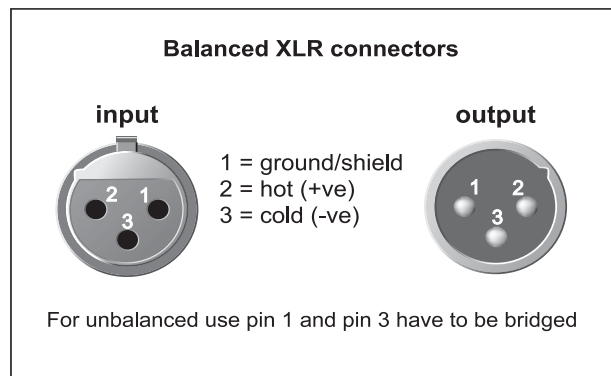
Fig. 4.2: XLR connector
