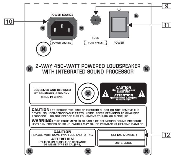
Fig. 2.2: Control elements and connections (B212A and B215A)
