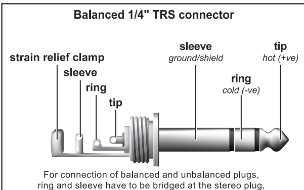
Fig. 4.1: 1/4" TRS connector
