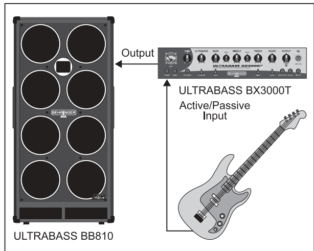
Fig. 3.3: Setup with the BB810 and the BX3000T
