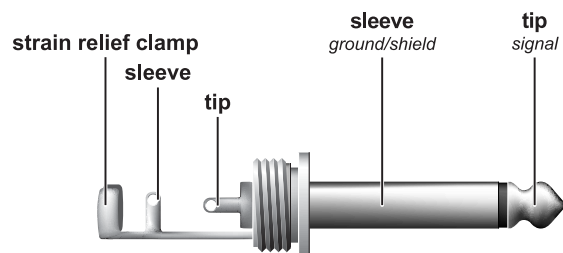
Fig. 4.3: 1/4" TS connector
