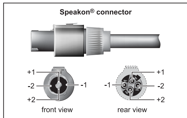
Fig. 4.1: Speakon® connectors
