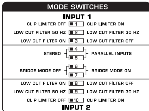
Fig. 2.3: DIP-switches
