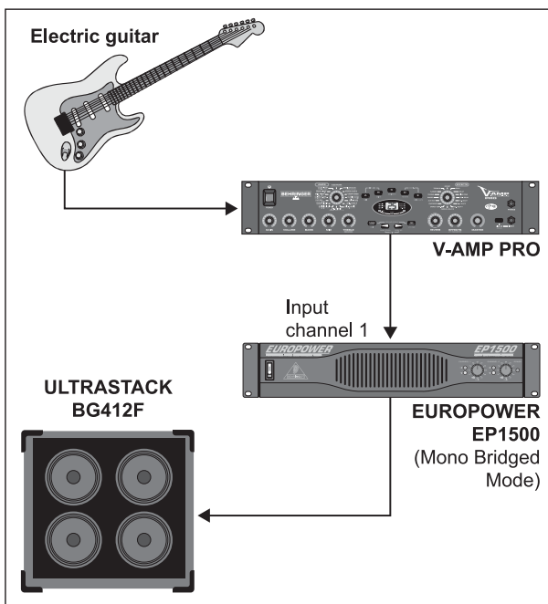
Fig. 3.5: Mono-bridged mode
