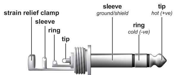
Fig. 4.4: 1/4" TRS connector
