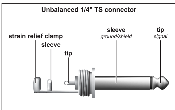
Fig. 4.2: 1/4" TS connector
