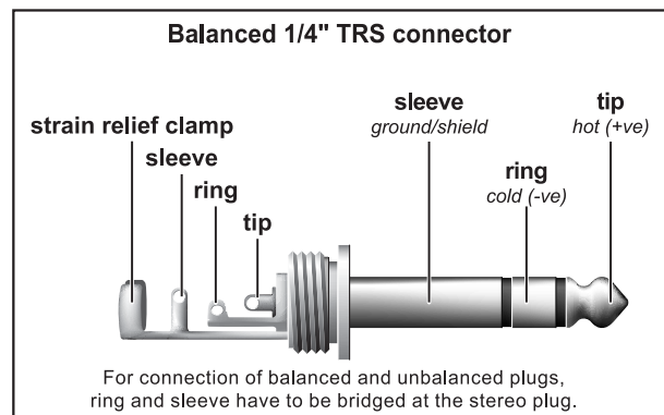
Fig. 4.3: 1/4" TRS connector
