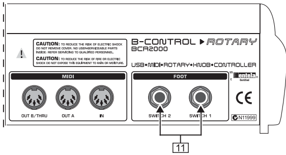
Fig. 3.3: The footswitch connectors on the BCF2000
