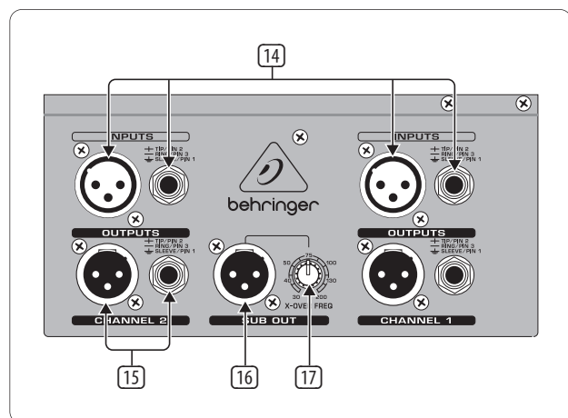
Fig. 2.3: Connectors at the rear of the FBQ3102
