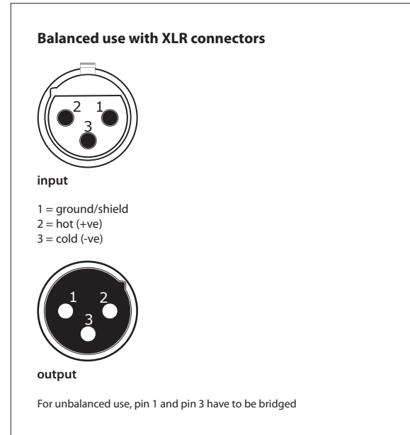
Fig. 4.2: XLR connections
