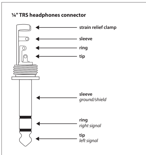
Fig. 4.5: ¼" TRS connector for headphones
