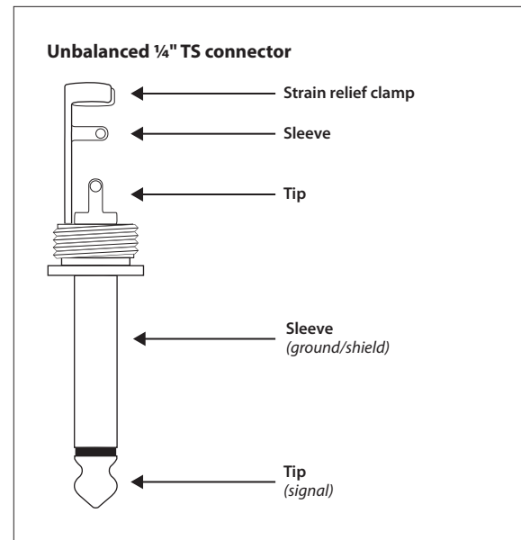
Fig. 4.3: 1/4" TS connector
