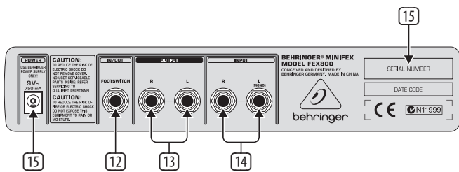
Fig. 2.2: Rear panel connectors of the FEX800
