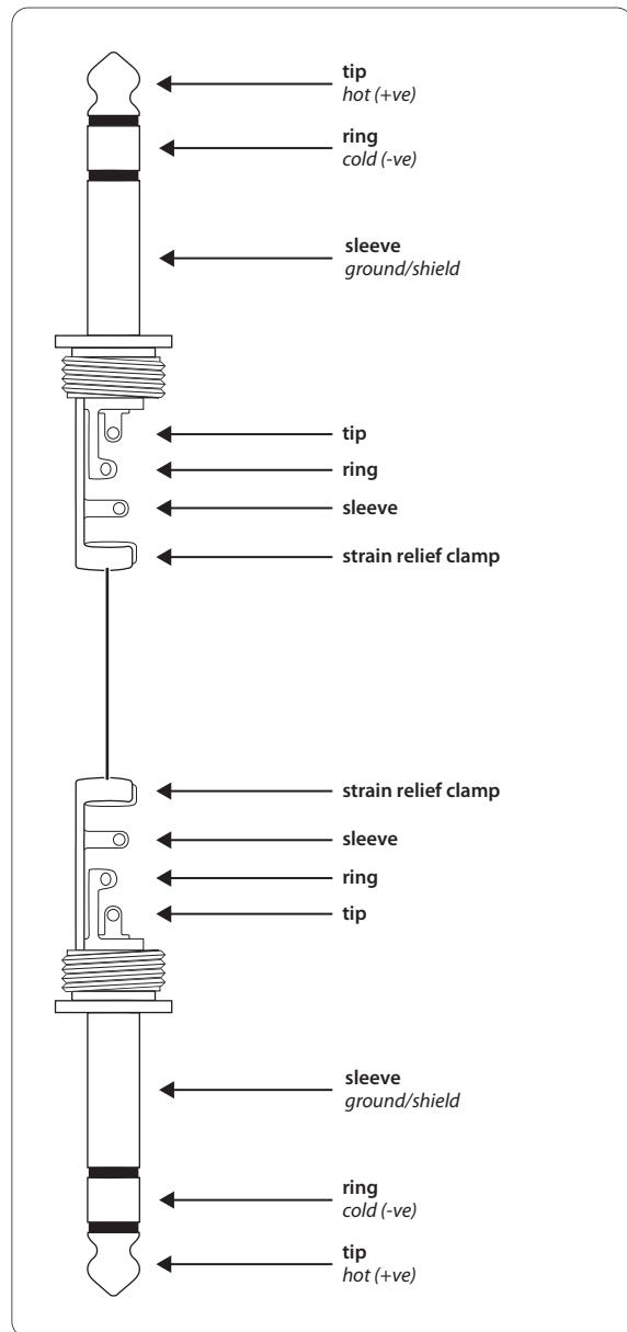
Fig. 5.2: Unbalanced cable with 1/4" TS connectors
