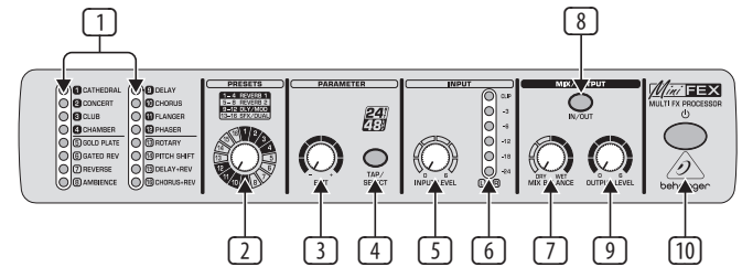
Fig. 2.1: Front panel control elements of the FEX800
