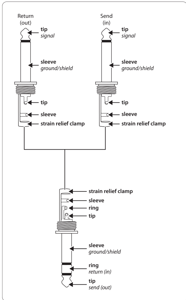
Fig. 5.1: Insert cable with two 1/4" TS and one 1/4" TRS connector
