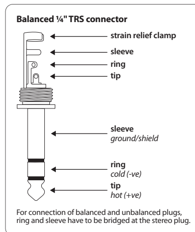
Fig. 4.2: Balanced jack cable with 1/4" TRS jack plugs
