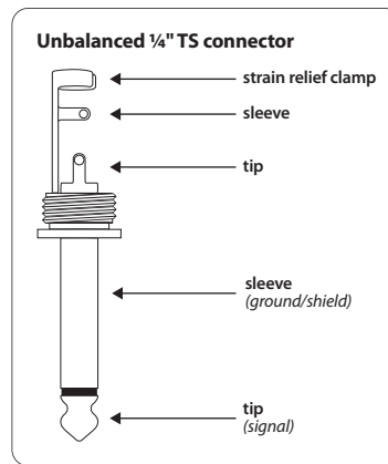
Fig. 4.1: Unbalanced jack cable with 1/4" TS jack plugs
