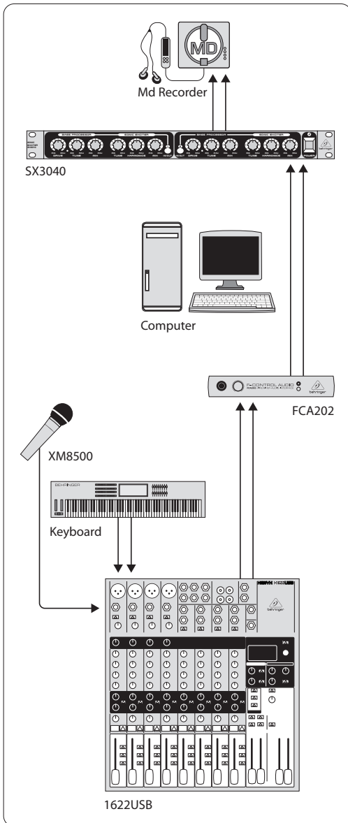
Fig. 3.2: The SX3040 in Studio mode
