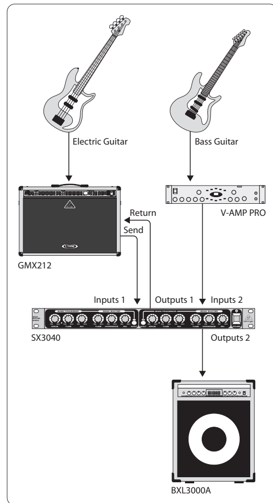
Fig. 3.3: The SX3040 in use with guitar amplifiers
