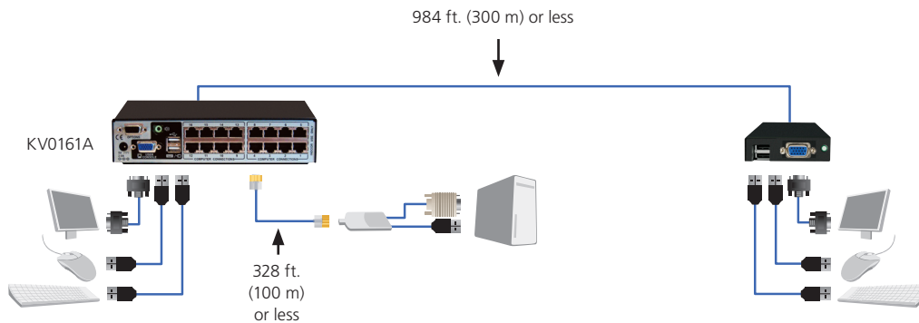
Figure 3-1. Application diagram #1.
