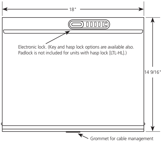
Figure 3-1. Front view.
