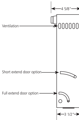
Figure 3-2. Side view.
