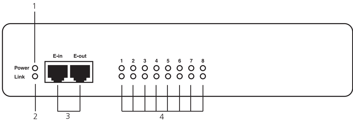
Figure 2-1. Front panel.
