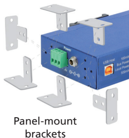
Figure 4. Panel-mount bracket positions.
