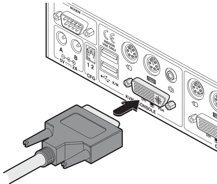
Analogue video link
