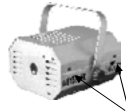
Remove screws on both sides.
