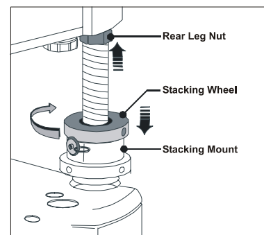
Figure 10. Secure Hardware
