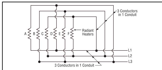
Figure 7 — Delta Connection
