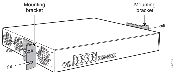
Figure 1-3 Mid-Mounting the Brackets on the CSS 11050 and CSS 11150
