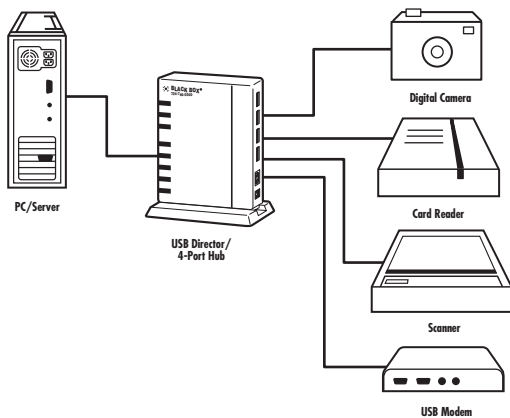
Figure 2-2. Typical Application.
