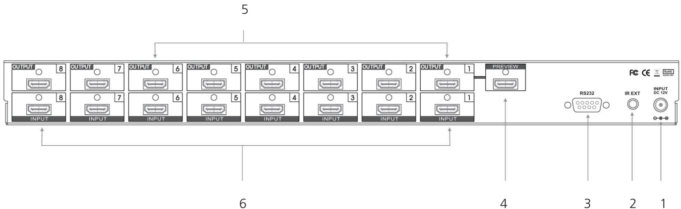
Figure 2-3. Rear panel.
