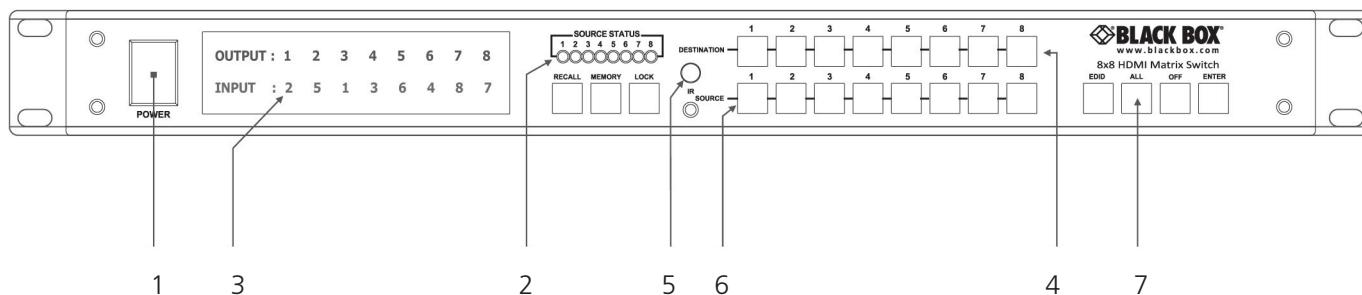
Figure 2-1. Front-panel diagram #1.
