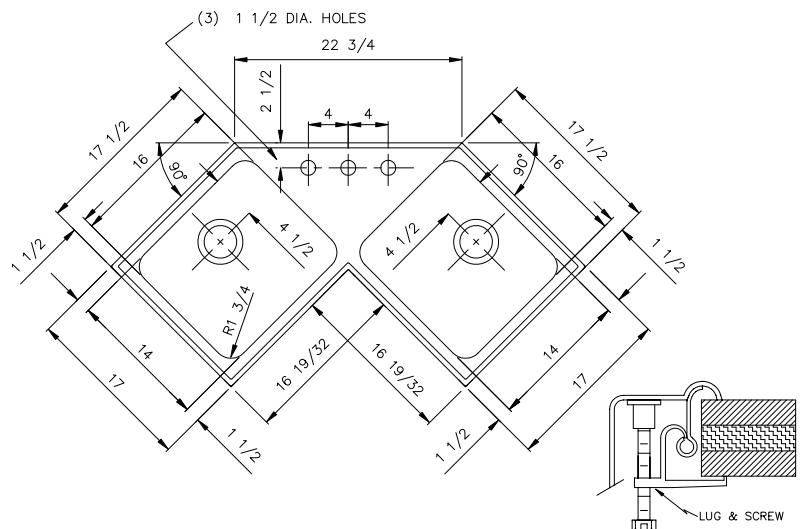
SECTION THRU FLANGE MAKE CUTOUT ACCURATELY, 3/4 LESS IN WIDTH AND IN LENGTH THAN OVERALL SIZE. CORNERS OF CUTOUT MAY BE SQUARE OR ANY RADIUS UP TO 1/2.
