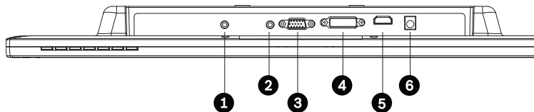
Figure 3.2 Bottom View (I/O Panel)
