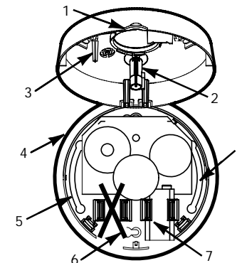
Parts of Smoke Alarm (Cover Open)
