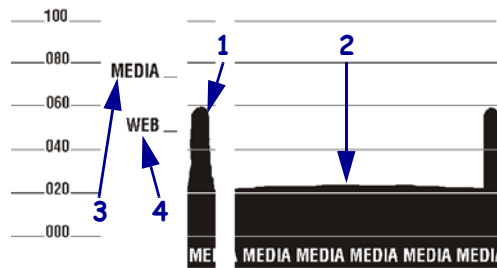
Figure 43 • Sensor Profile (Media Section)
