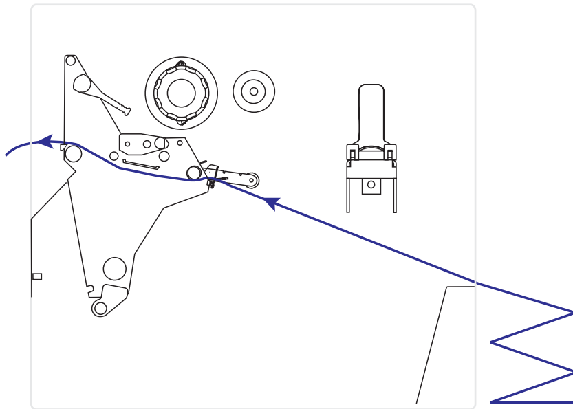
Figure 16 • Rear Feed Using Media Supply Hanger
