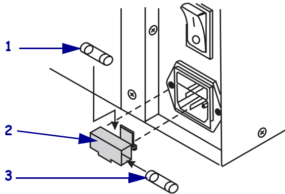
Figure 37 • Fuse Locations
