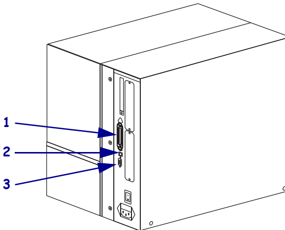
Figure 5 • Cable Connections
