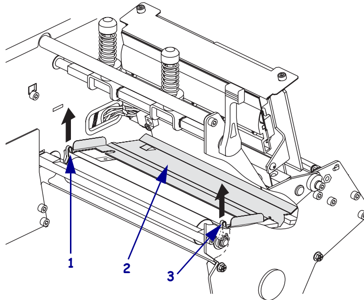
Figure 35 • Snap Plate
