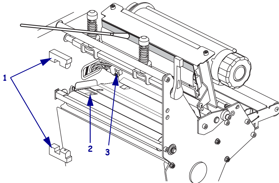
Figure 32 • Sensor Locations
