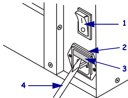
Figure 36 • AC Power Entry Module
