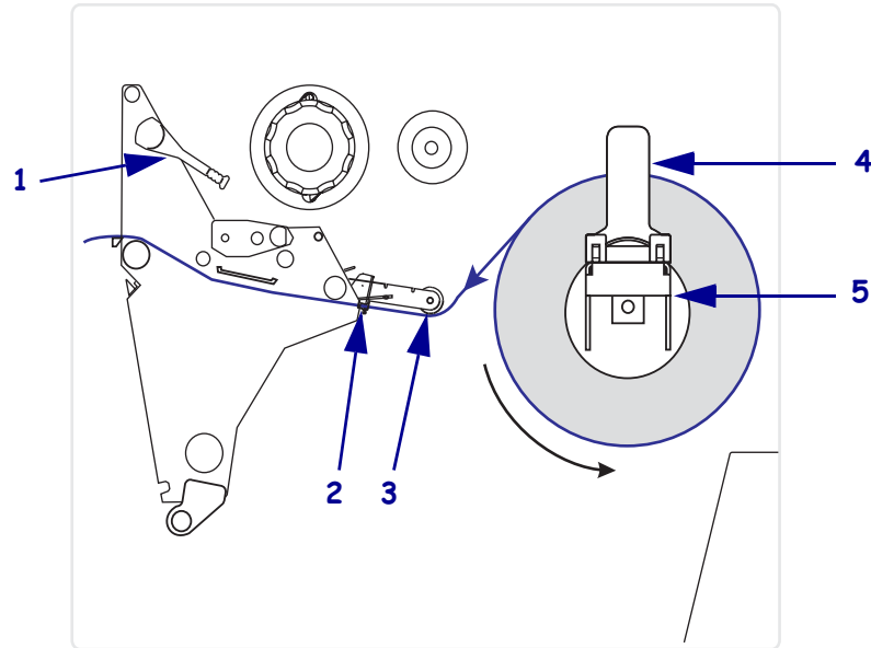
Figure 18 • Tear-Off Mode
