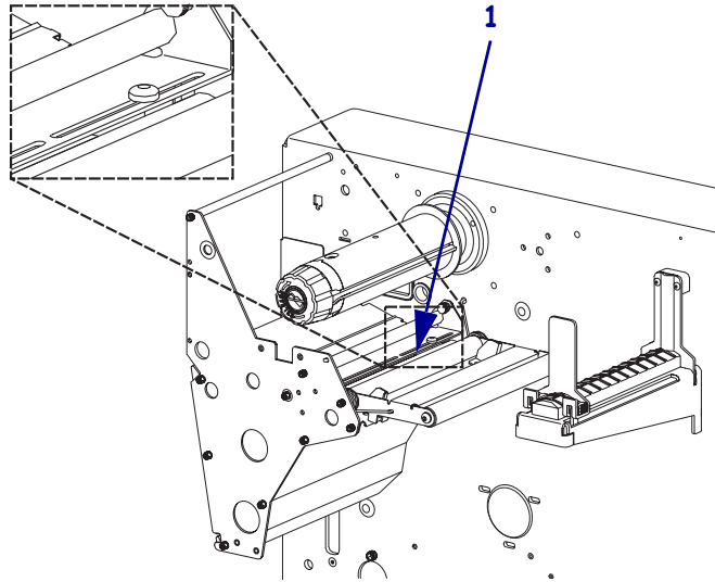
Figure 33 • Upper Media Sensor
