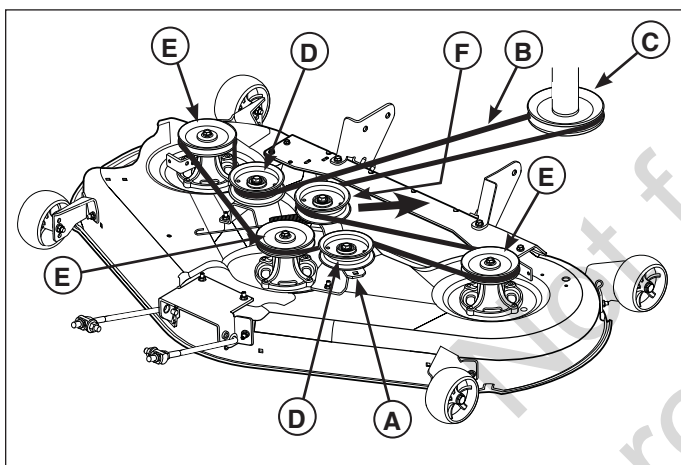
Figure 18. Mower Belt Routing
