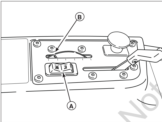
Figure 16. Cutting Height Adjustment
