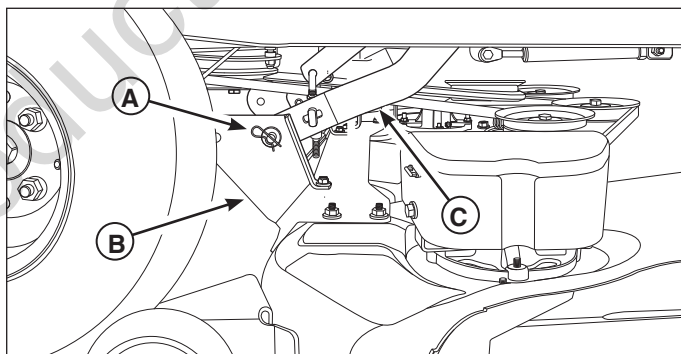
Figure 19. Rear Deck Lift Components (Right side shown, left side same)
