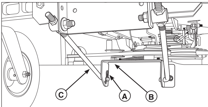
Figure 20. Front Deck Lift Components (Right side shown, left side same)
