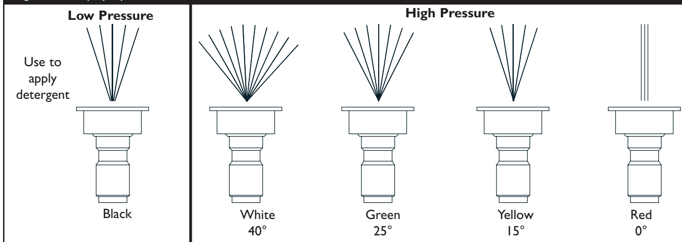
Figure 10 — Spray Tips
