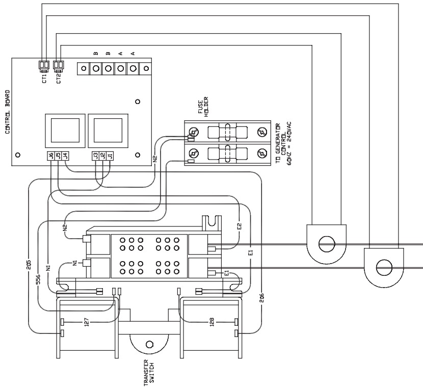
WIRE DIAGRAM
