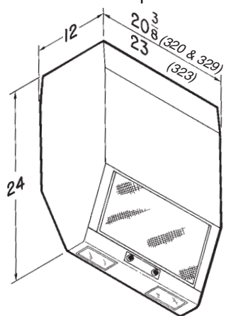
Model 320 Interior Blower (420 cfm) Model 323 Interior Blower (1170 cfm) Model 329H Interior Control Pack (for use with Models 331H & 332H)
