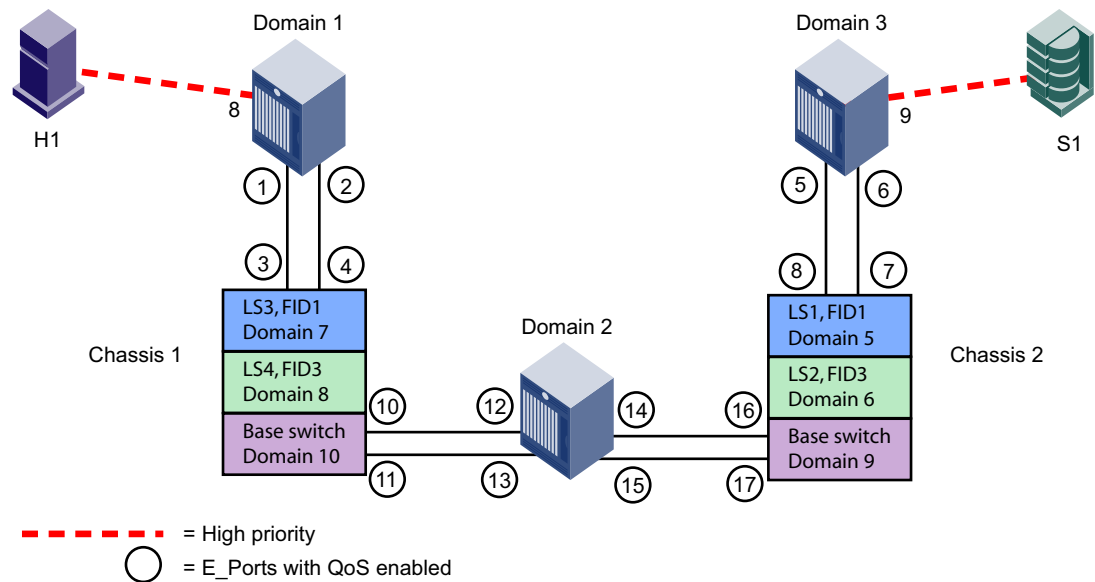
FIGURE 63 Traffic prioritization in a logical fabric
