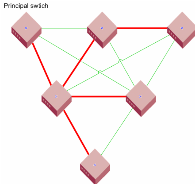
FIGURE 5 Principal ISLs
