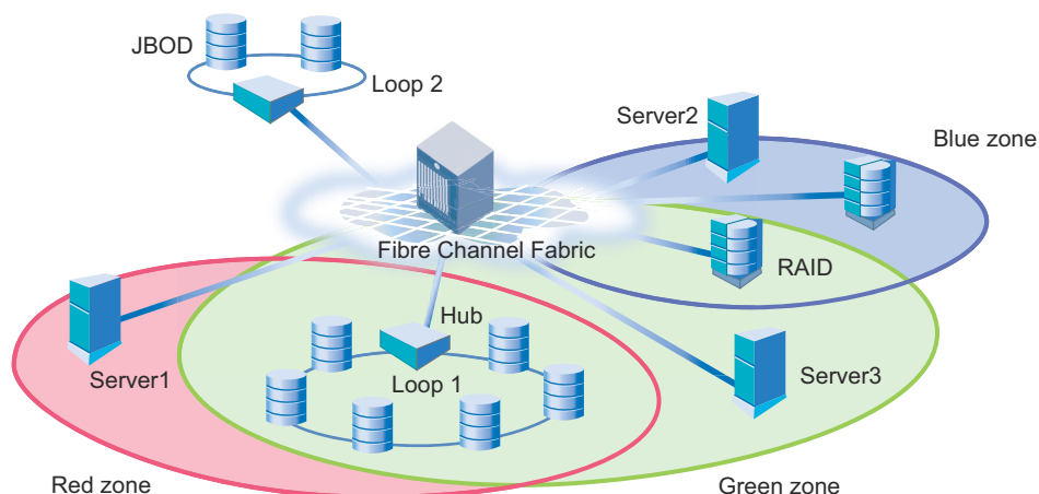
FIGURE 32 Zoning example
