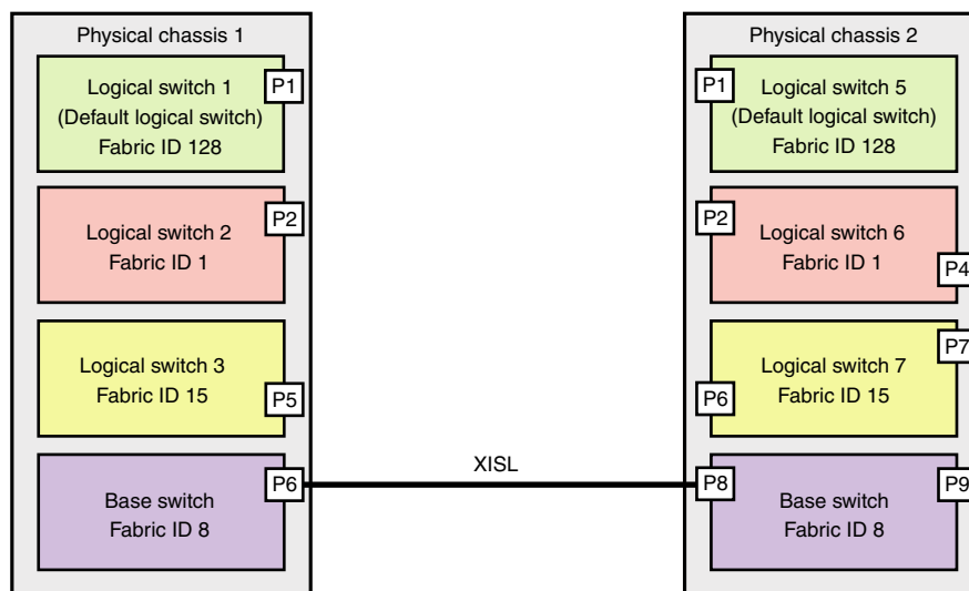
FIGURE 28 Base switches connected by an XISL
