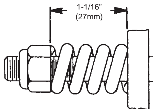
Figure 4-9 Clutch Spring Length
