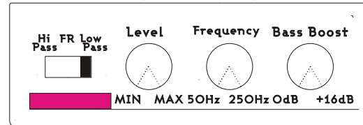
Q Series two channel crossover section, located under the light up plastic plate.
