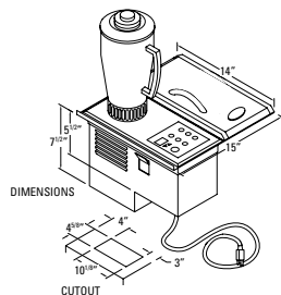
TOP COUNTER BLENDER COVER
