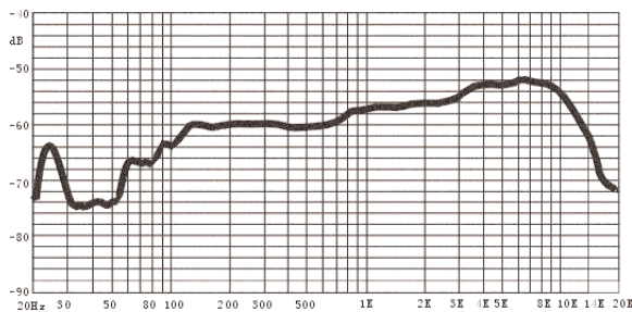
Frequency Response PADM-510
