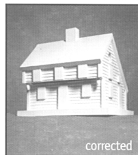
1. Tilt the camera backward to the horizontal position to correct the perspective. 2. Shift the camera front panel upwards to position the subject in the right position and refocus if necessary.
