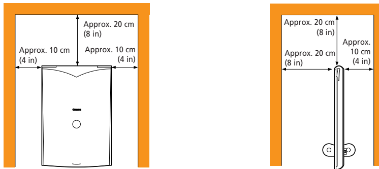
Scanner in a vertical position
