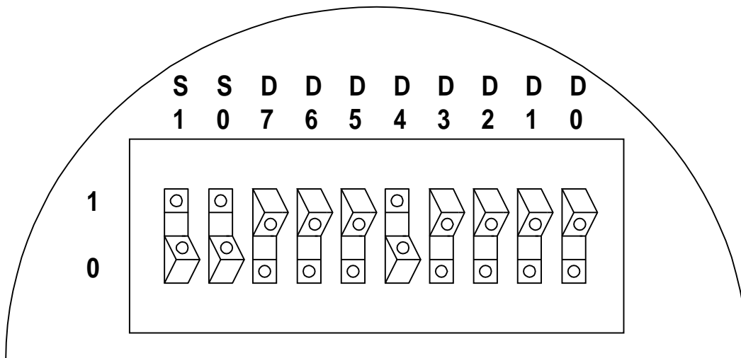
Figure 3. Dip Switches Set to Value 1100010000 to Reset the XRD9829
