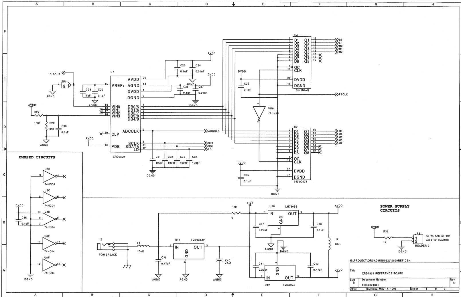
Schematics for XRD9829REF Page 1 of 3.
