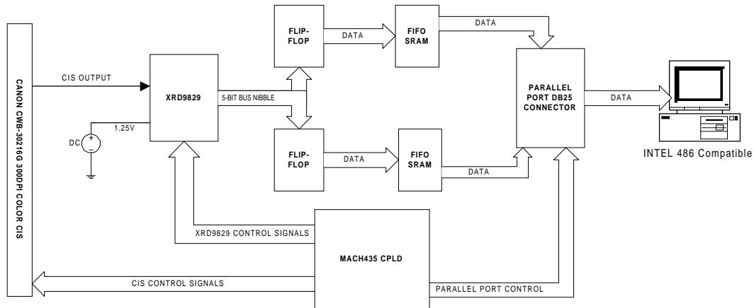
Figure 1. Block Diagram of XRD9829REF
