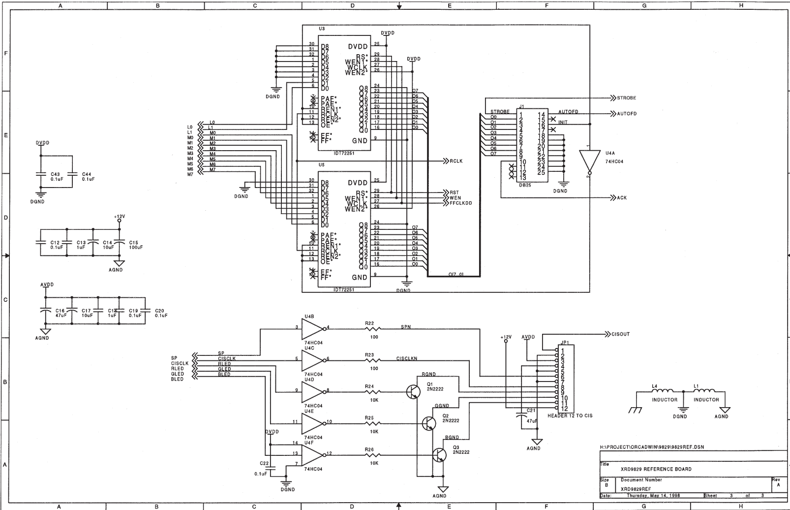
Schematics for XRD9829REF Page 3 of 3.
