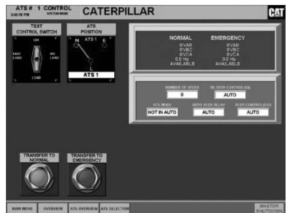
Screenshot of ATS operating parameters on Cat Switchgear HMI.
