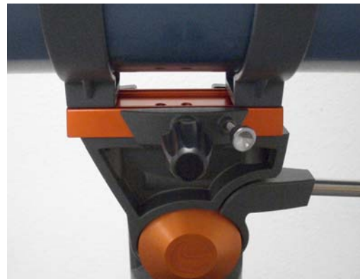
Figure 2-12 Mounting Knob & Safety Screw in the dovetail bracket. Shown is the 90AZ telescope tube
