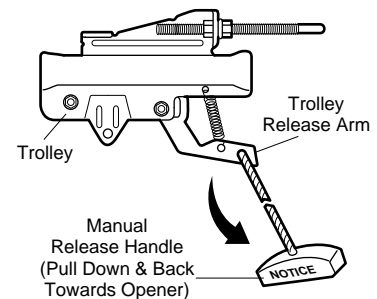
Lockout position
