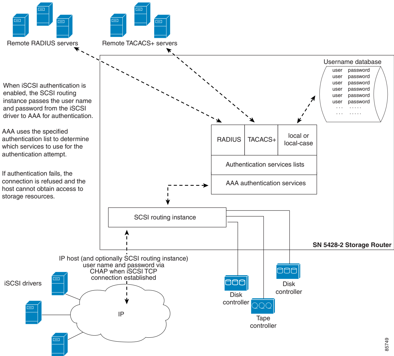
Figure 9-1 iSCSI Authentication Configuration Elements
