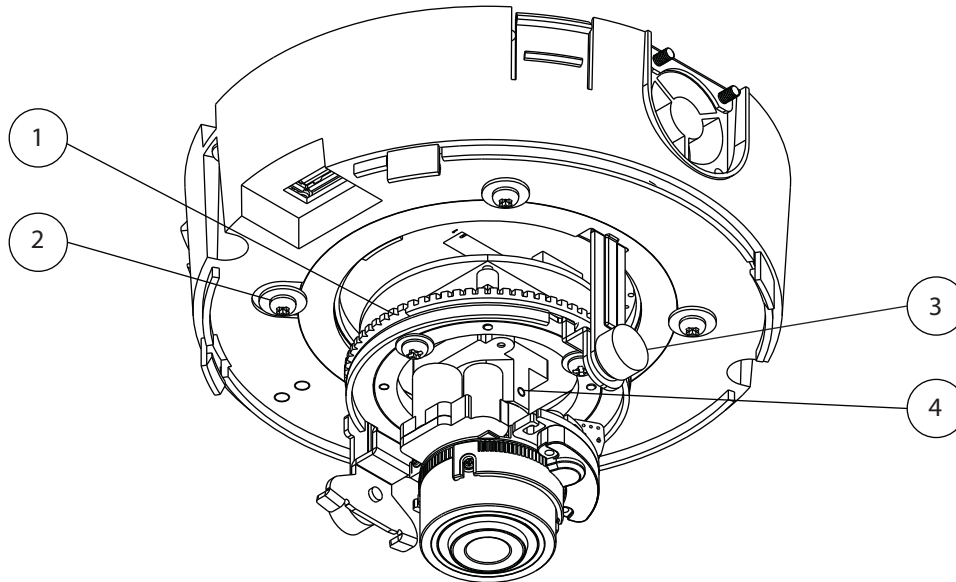
Figure 2-13 Adjusting the Camera Lens on the 2630 IP Dome
