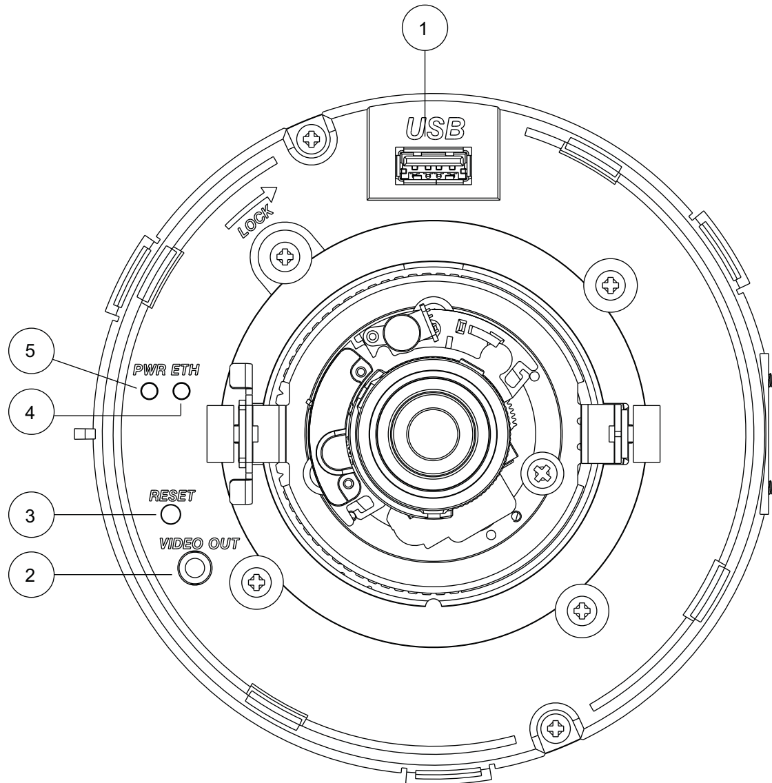
Figure 1-2 Bottom of the 2630 IP Dome
