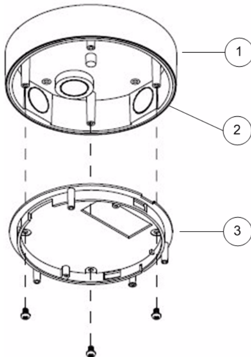
Figure 2-4 Attaching Base Plate to Conduit Base
