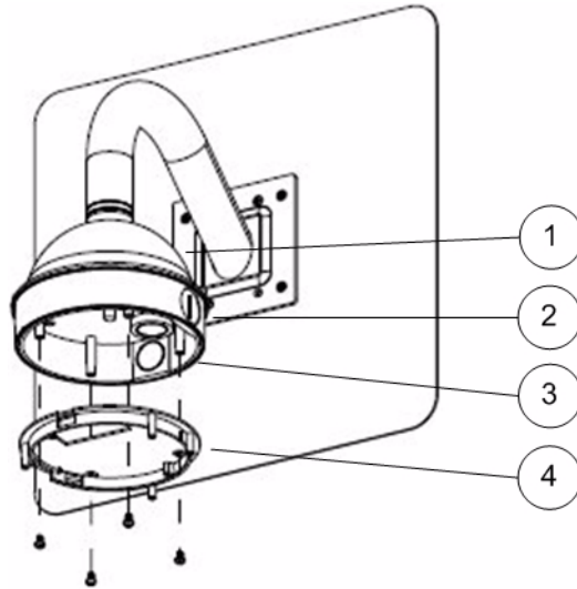
Figure 2-10 Attaching the Base Plate to the Conduit
