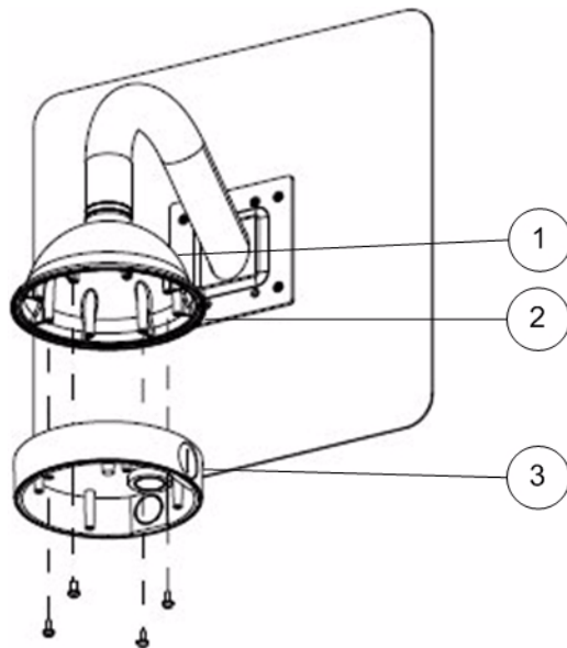
Figure 2-9 Attaching the Conduit Base to the Pendant
