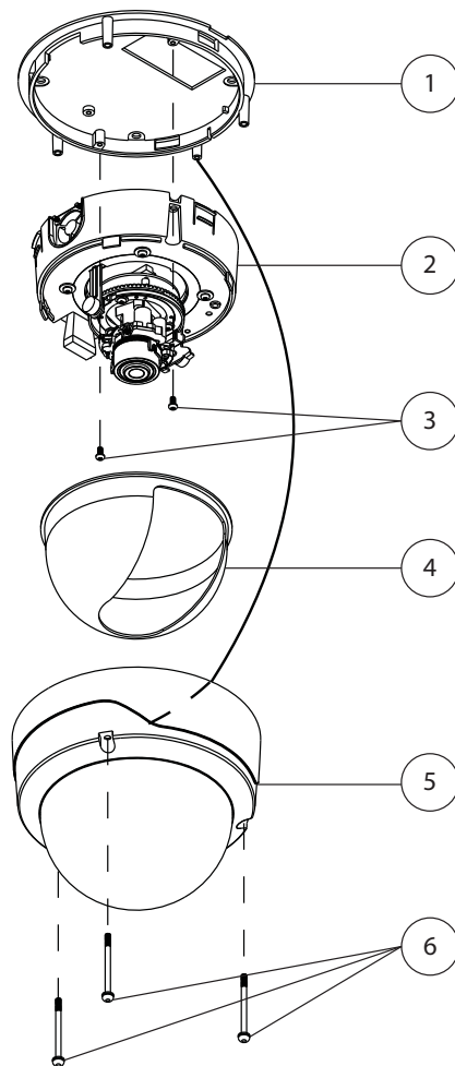
Figure 2-2 Disassembling the 2630 IP Dome Components
