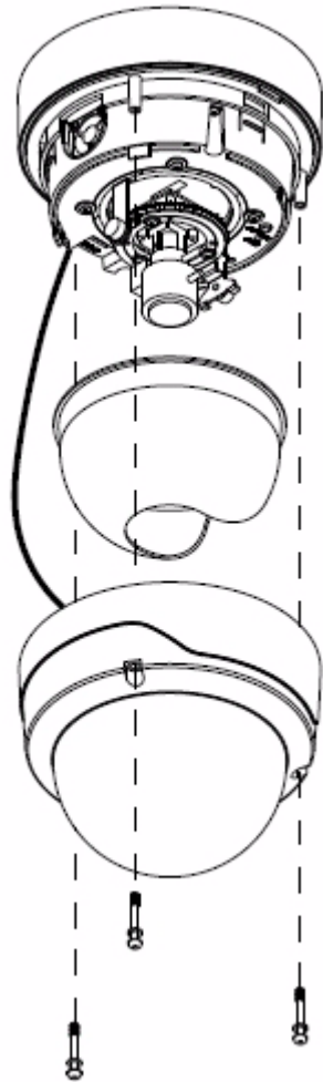
Figure 2-6 Attaching the Privacy Shield and Dome
