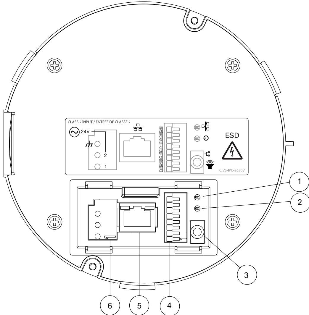
Figure 1-1 Top of the 2630 IP Dome
