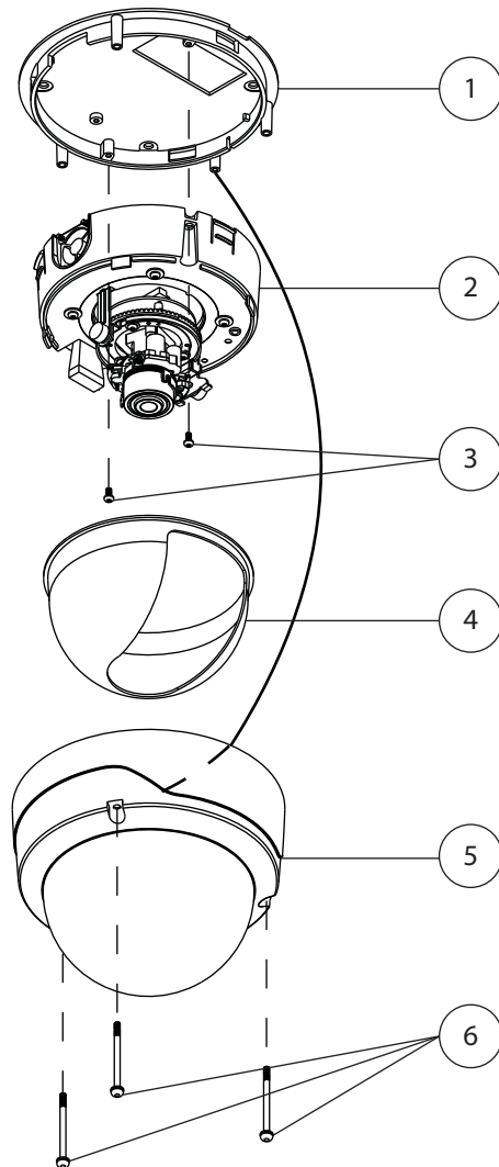
Figure 2-7 Disassembling the 2630 IP Dome Components
