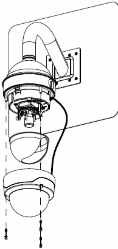
Figure 2-12 Attaching the Privacy Shield and Dome
