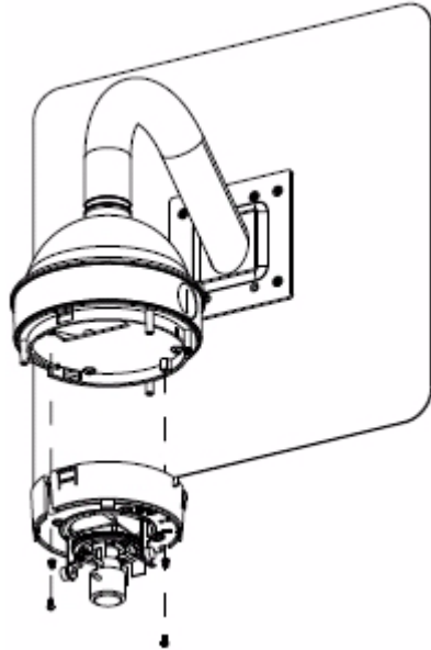
Figure 2-11 Attaching the Camera to the Base Plate
