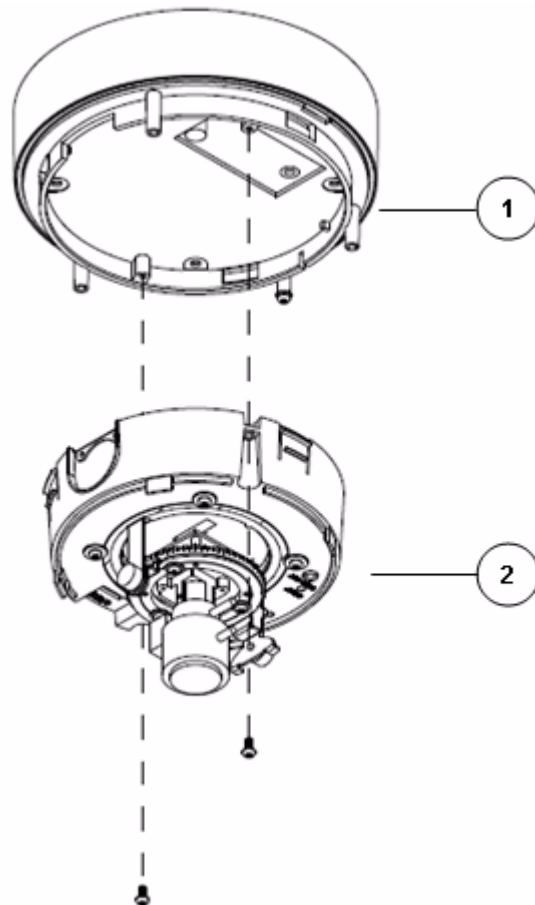
Figure 2-5 Attaching the Camera to the Base Plate
