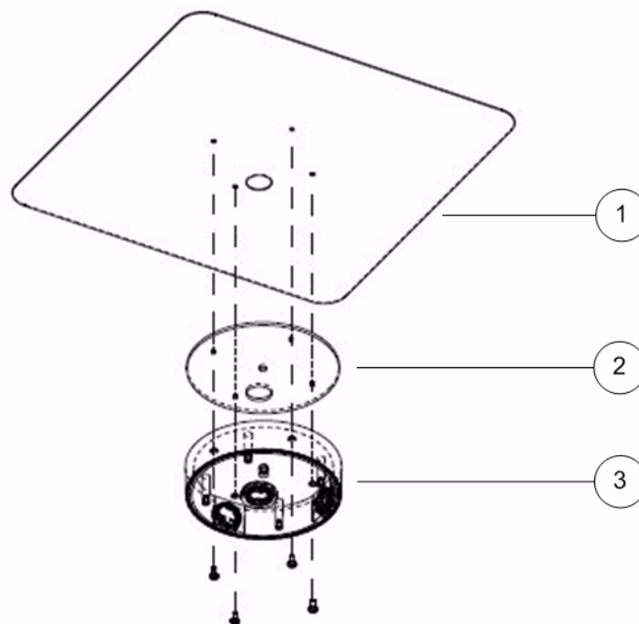
Figure 2-3 Attaching the Conduit Base to a Ceiling or Wall
